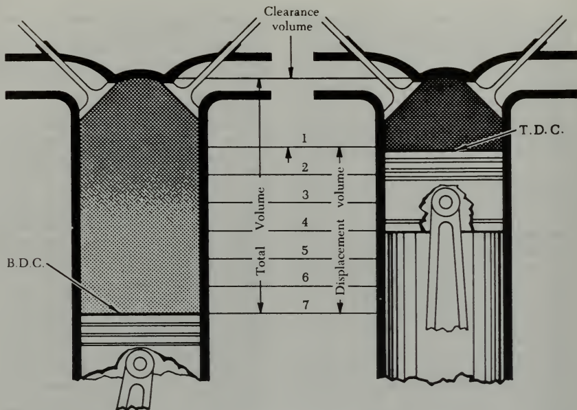
FIGURE 1-27. Compression ratio.
